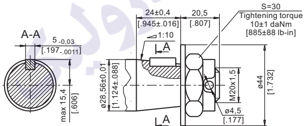
K - tapered 1:10, Parallel key B5x5x14 DIN 6885 Max. Torque 40 daNm [3540 lb-in]
