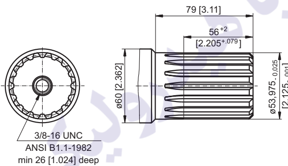
S - \phi 2\frac{1}{8} " [53,975] splined 16 DP 8/16 ANS B92.1-1976
