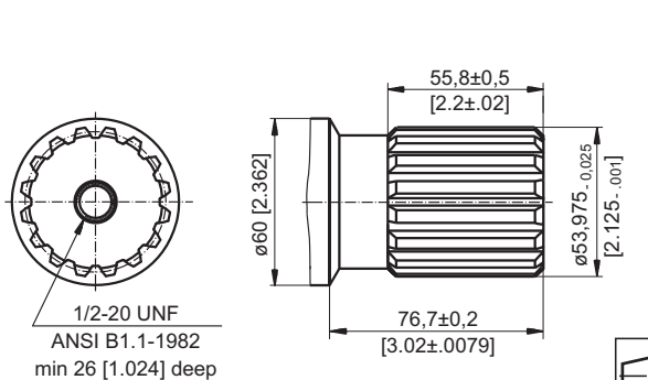
S - \phi 2\frac{1}{8} " [53,975] splined 16 DP 8/16 ANS B92.1-1976
