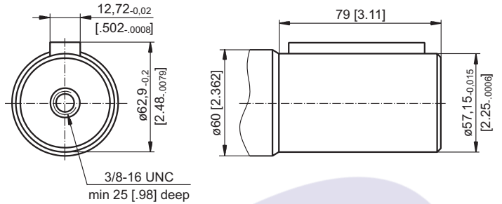
B - \phi 2\frac{1}{4} " [57,15] straight Parallel key \frac{1}{2} "x \frac{1}{2} "x 2\frac{1}{4} " BS46
