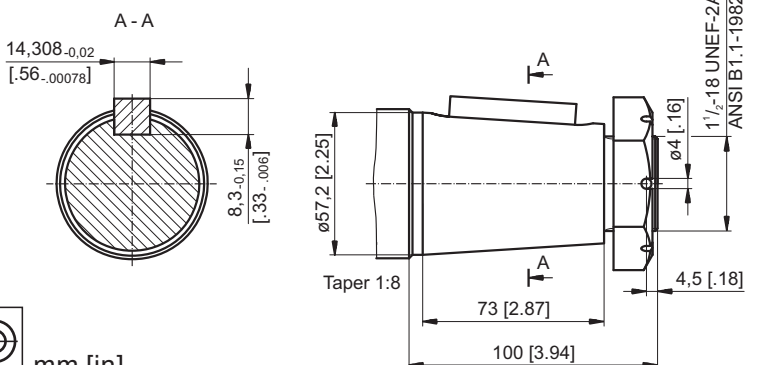
T - \phi 2\frac{1}{4} " [57,15] SAE J501, tapered 1:8 key \frac{9}{16} "x \frac{9}{16} "x2" BS46
