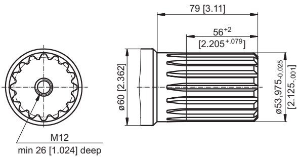
SH - \phi 2\frac{1}{8} " ( \phi 53,975 ) splined 16 DP 8/16 ANS B92.1-1976
